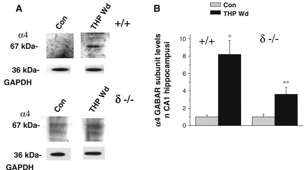
Fig. 2 Withdrawal from THP increases \alpha 4 subunit expression. THP withdrawal (THP Wd) in both +/+ and \delta -/- mice increased expression of the \alpha 4 subunit in isolated CA1 hippocampal membranes, without altering levels of the GAPDH control protein. a Representative Western blot. b Group means. ( *P < 0.05 vs Con, n = 9 animals, each)
